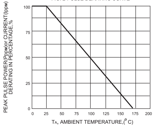
FIG. 2-PULSE DERATING CURVE
