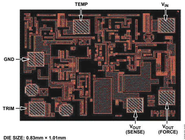
Figure 3. Die Layout
