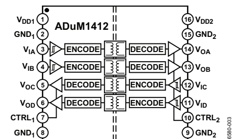
Figure 3. ADuM1412
