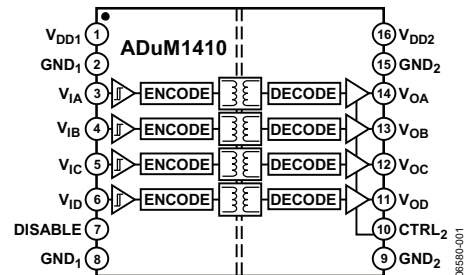
Figure 1. ADuM1410
