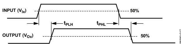
Figure 17. Propagation Delay Parameters
