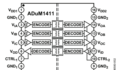
Figure 2. ADuM1411
