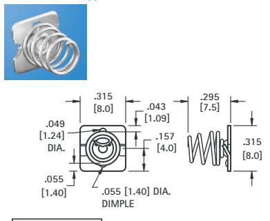
(-) NEGATIVE SPRING
