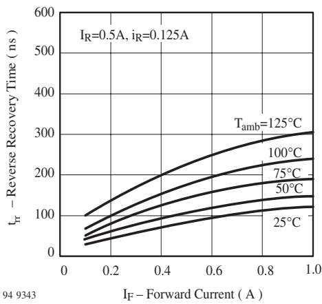
Figure 6. Max. Reverse Recovery Time vs. Forward Current
