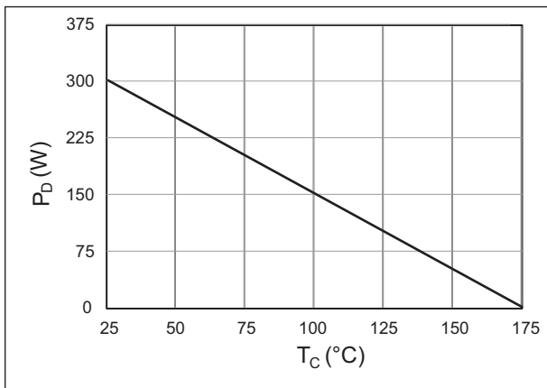
Power Derating
