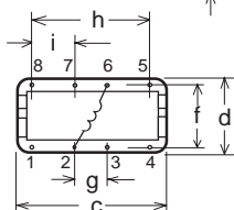
Type F - Flat Mount
