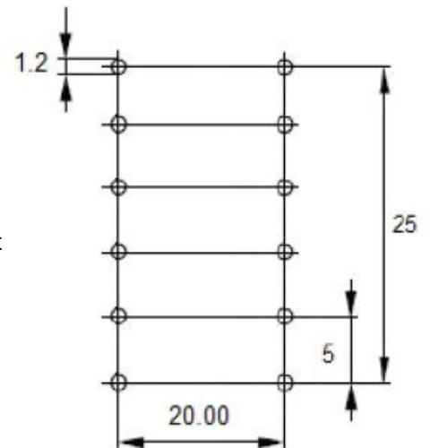
Hole arrangement View in mounting
