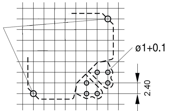
Hole arrangement View in mounting direction
