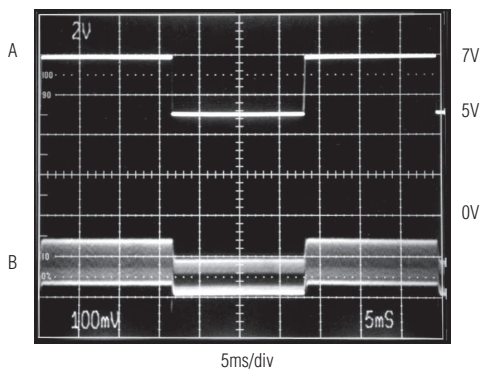
LINE-TRANSIENT RESPONSE
