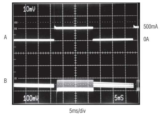
LOAD-TRANSIENT RESPONSE
