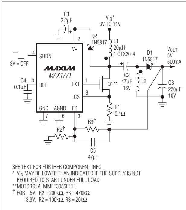
Figure 5. Step-Up/Down for a 5V/3.3V Output
