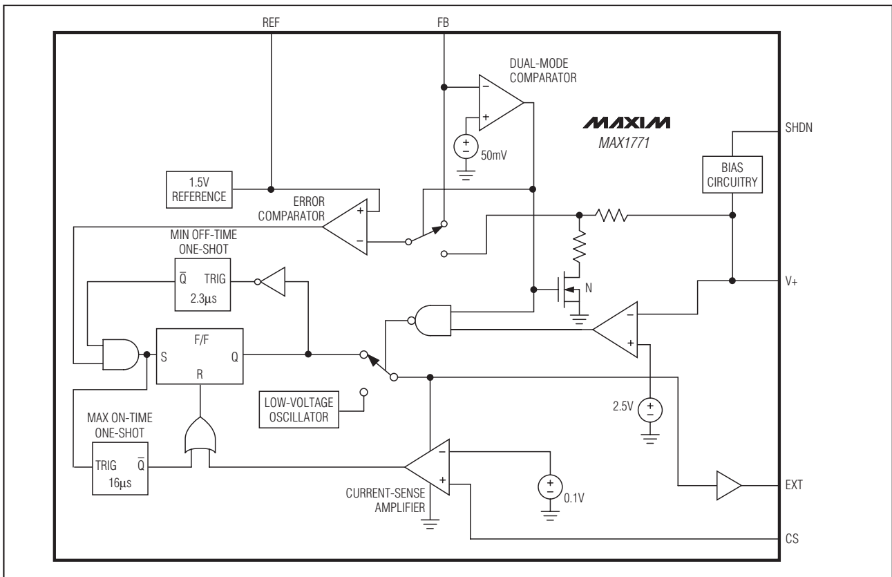
Figure 1. Functional Diagram
