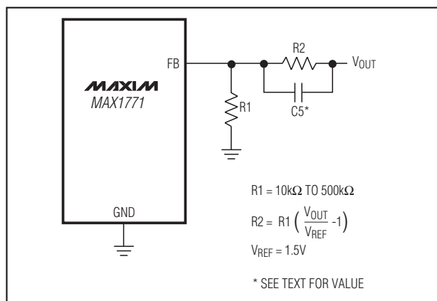
Figure 3. Adjustable Output Circuit
