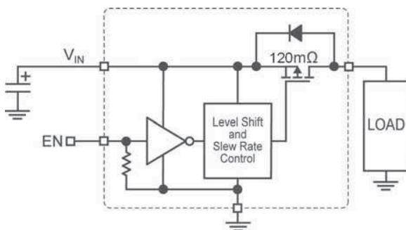
MIC94070, 72 Load Switch Application
