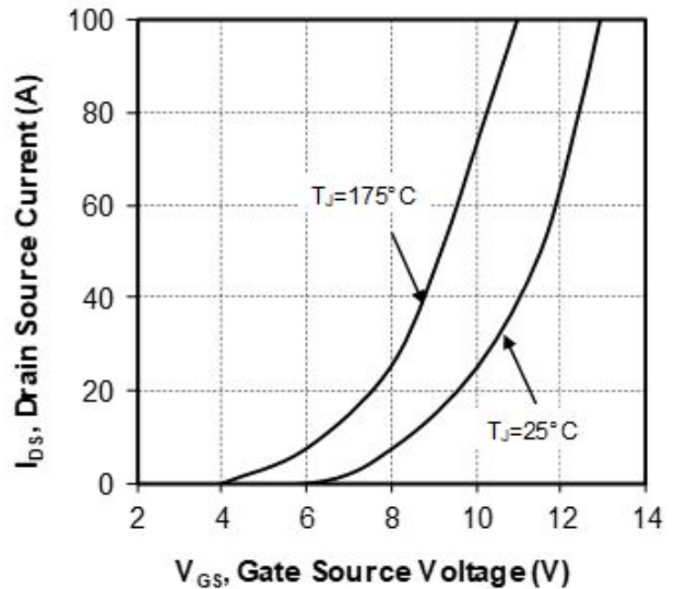
Figure 1-5. Transfer Characteristics
