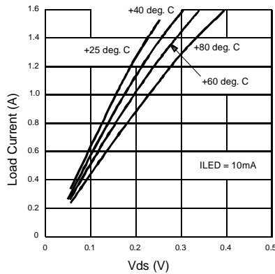
Figure 3. Typical On-Characteristics
