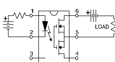
"B" Connection
