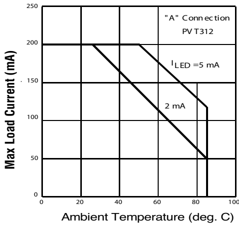
Figure 1. Typical Current Derating Curves
