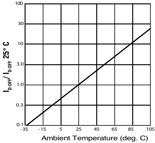
Figure 5. Typical Normalized Off-State Leakage
