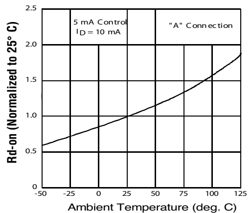
Figure 4. Typical Normalized On-Resistance
