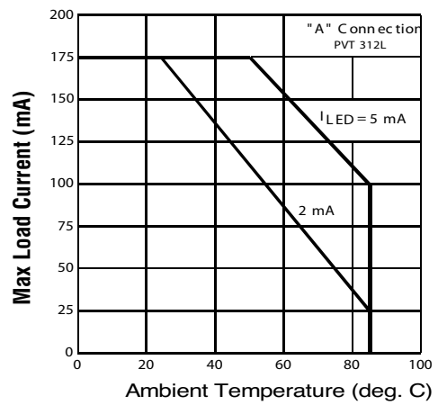
Figure 2. Typical Current Derating Curves
