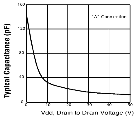
Figure 9. Typical Output Capacitance
