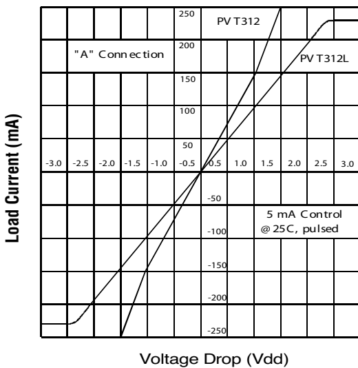
Figure 3. Linearity Characteristics
