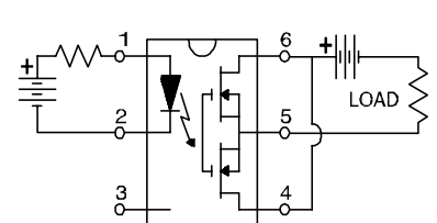
"C" Connection
