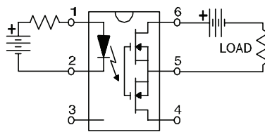
"B" Connection
