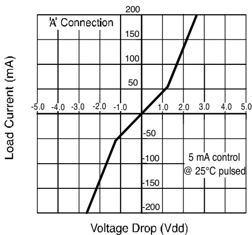
Figure 3. Linearity Characteristics
