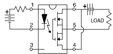
"C" Connection
