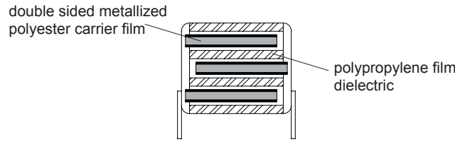
1 section (250Vdc)
