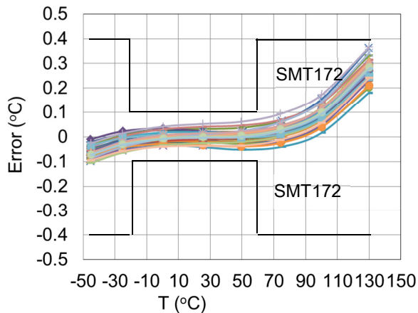
Accuracy vs. temperature ( V_{CC}=5V , TO18)
