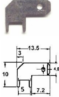
FASTON 4.8 VL LS1537
