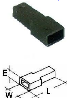
FASTON 4.8 kryt KKM
