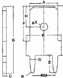
FASTON 4.8 V 805203BL
