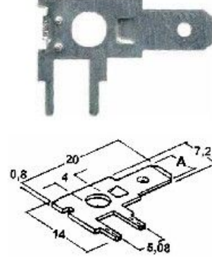
FASTON 4.8 VL CC648 Sn
