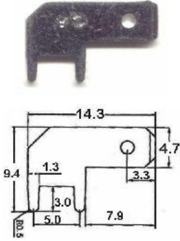
FASTON 4.8 VL 805212BL
