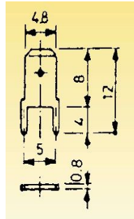
FASTON 4.8 V CC341 Sn
